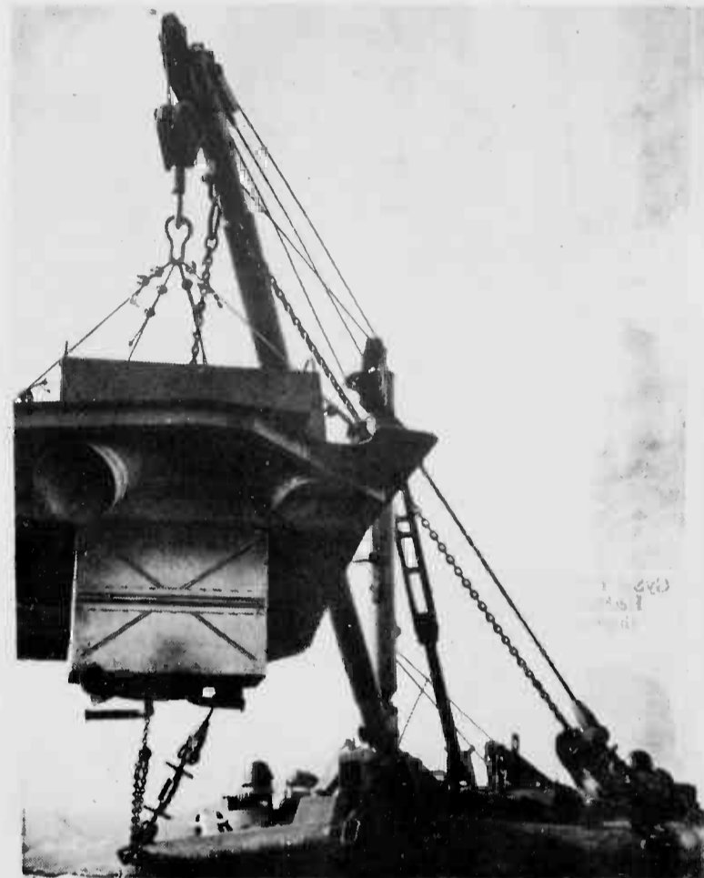
"THE DOGHOUSE", better known as an air intake and exhaust superstructure, fits above the engine in an AMTRAC and is here being lifted by the LVTR1 repair vehicle.
